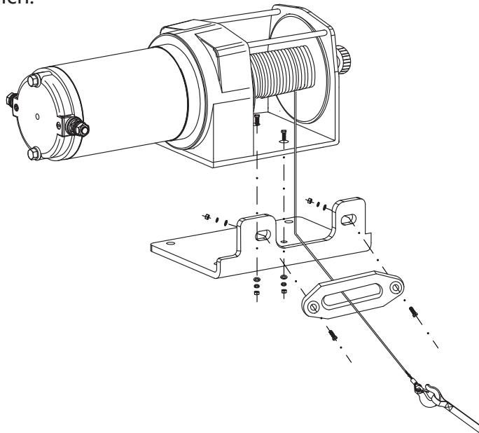
Fig. 2 - Winch mounting
